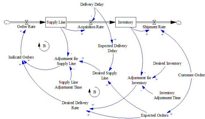
System dynamics modeling
